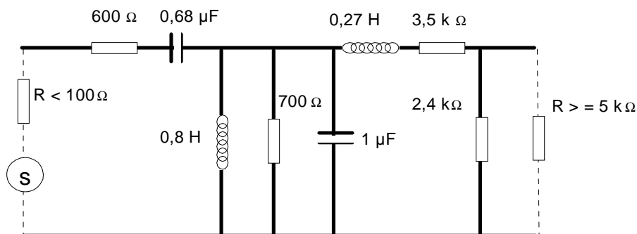
Figure 2: Filter circuit
